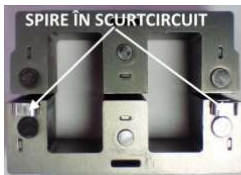
Figura 3.35 Miezuri magnetice contactor electromagnetic.
